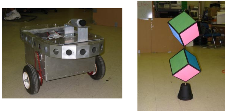
Figure 3: The CMU Deminer robot used in the experiment (left) and cube stack used to measure robot pose (right).
