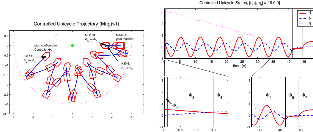
Figure 2: This figure depicts the simulated unicycle trajectory for an initial condition q_0 such that M(q_0) > 1 . The sequential composition starts in Controller \Phi_2 , then proceeds through \Phi_4 , \Phi_5 , and \Phi_7 before achieving the goal condition of \|q(t) - q_f\| < \epsilon .
