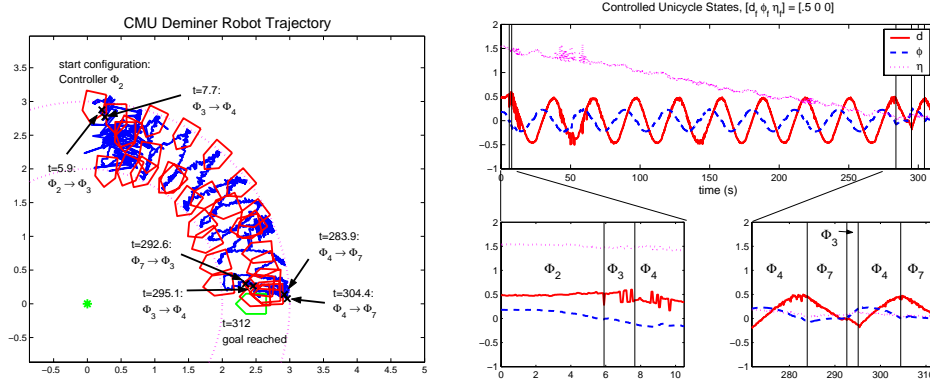
Figure 4: This figure depicts the trajectory of the CMU Deminer robot under sequential composition control. The figure on the left shows the trajectory of the robot in the plane, while the figure on the right shows the evolution of d , \varphi , and \eta . The sequential composition starts in Controller \Phi_2 , then proceeds through \Phi_3 , \Phi_4 , \Phi_7 , back to \Phi_3 , then to \Phi_4 and \Phi_7 before achieving the goal condition of \|q(t) - q_f\| < \epsilon = 0.06 .
