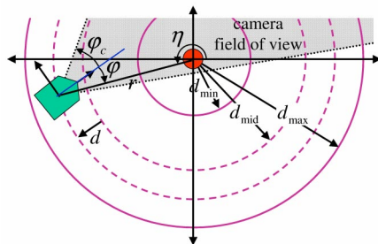
Figure 1: Unicycle coordinate system and camera configuration.
